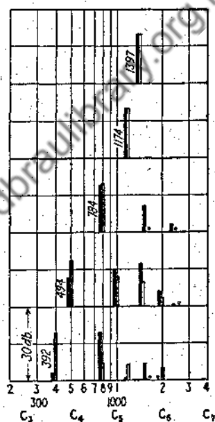
FIG. 7.—The flute.
