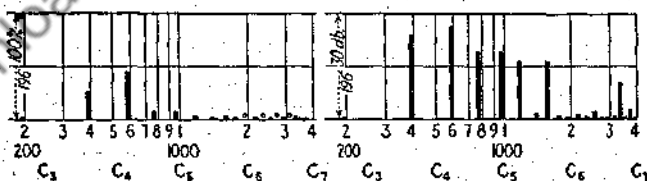
FIG. 2a.—Tone spectrum in terms of percentage of energy.
