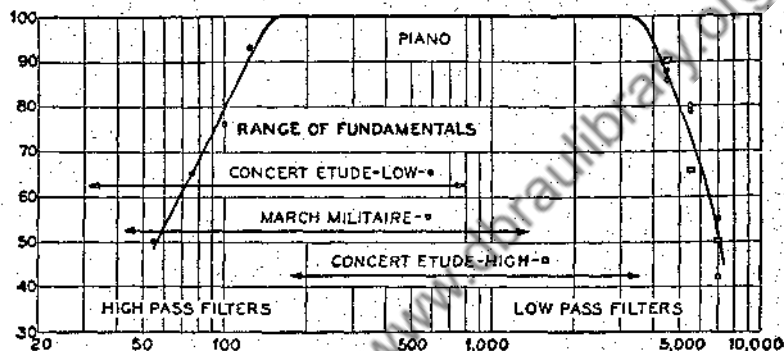
FIG. 3.—Number of times filter condition was correctly preserved as function of cutoff frequency for the piano. Figures at the bottom denote frequencies; figures at the left, per cent of correct judgments. The instrument was the piano. The range of the fundamentals for each selection is shown by the arrowed lines under the name of the selection. "High-pass filters" means that low frequencies were eliminated; "low-pass filters" means that high frequencies were eliminated. Thus in the Concert Etude , symbolized by a dot, the range was from 32 to 800~. For the March Militaire , symbolized by a circle, from 42 to 1,300~; and for the Concert Etude , symbolized by a square, from 192 to 2,500~. (Snow, 170 )
