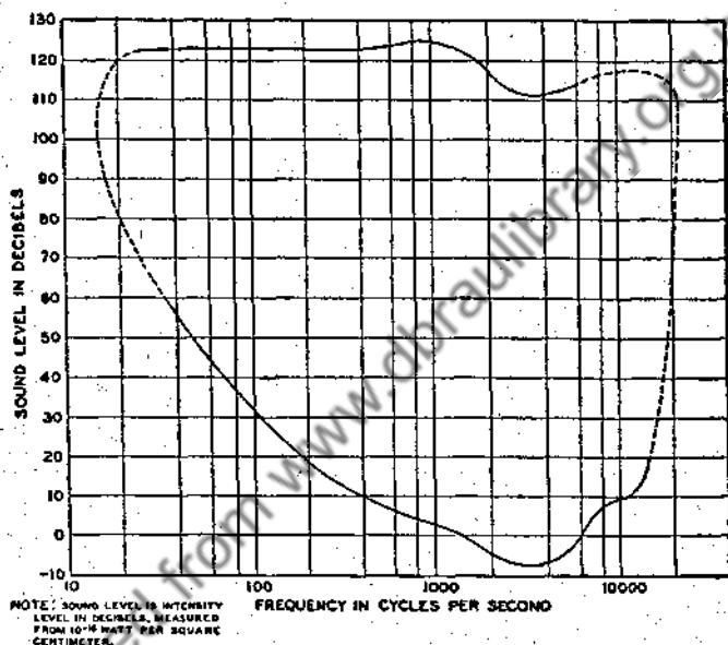
FIG. 2.—Limits of audible sound. (Courtesy of Western Electric Company.)
