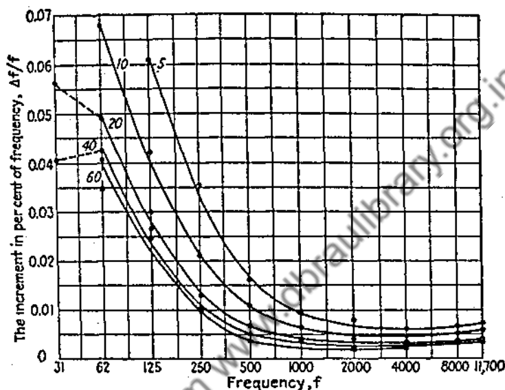
FIG. 1.—Variation with frequency level and sensation level. The numbers at the bottom denote frequency; at the side, the increment in per cent of frequency. The numbers within the figure denote sensation level, that is, number of db above the threshold of audibility. For example, for the frequency of 125~, the increment must be 6 per cent for a 5 db tone, 4 per cent for a 10 db tone, and between 2 and 3 per cent for 20, 40, and 60 db tones, respectively. ( Shower and Biddulph . 151 )
