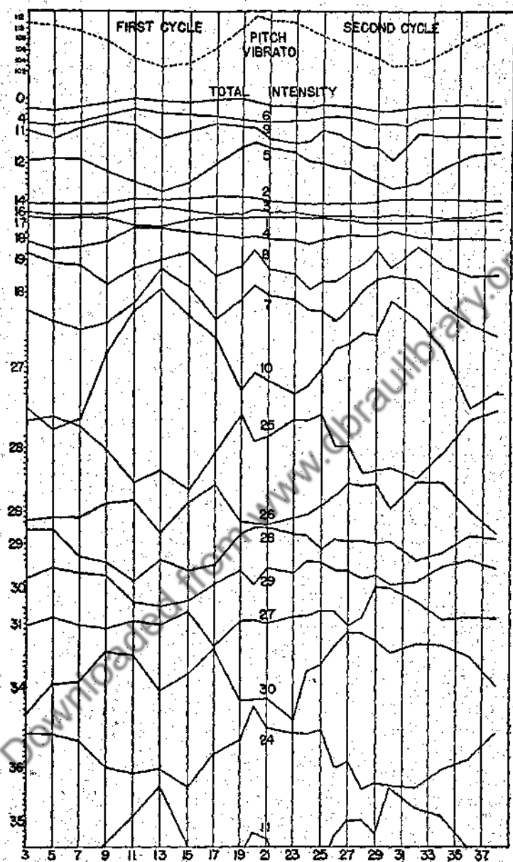
FIG. 2.—The harmonic structure of a beautiful tone. (Borchers. 9 )
