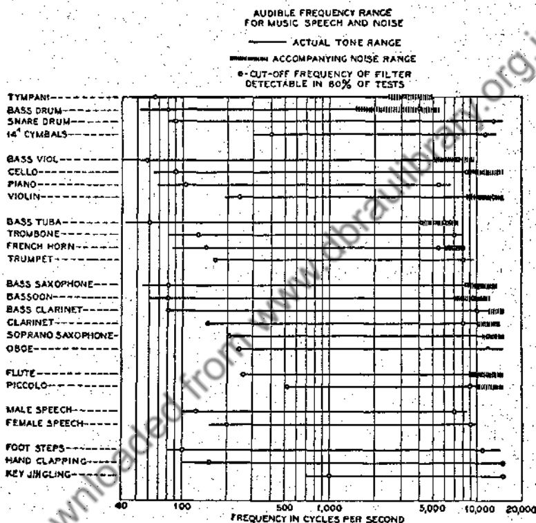
FIG. 4.—Audible frequency range for music, speech, and noise. ( Snow . 170 )
