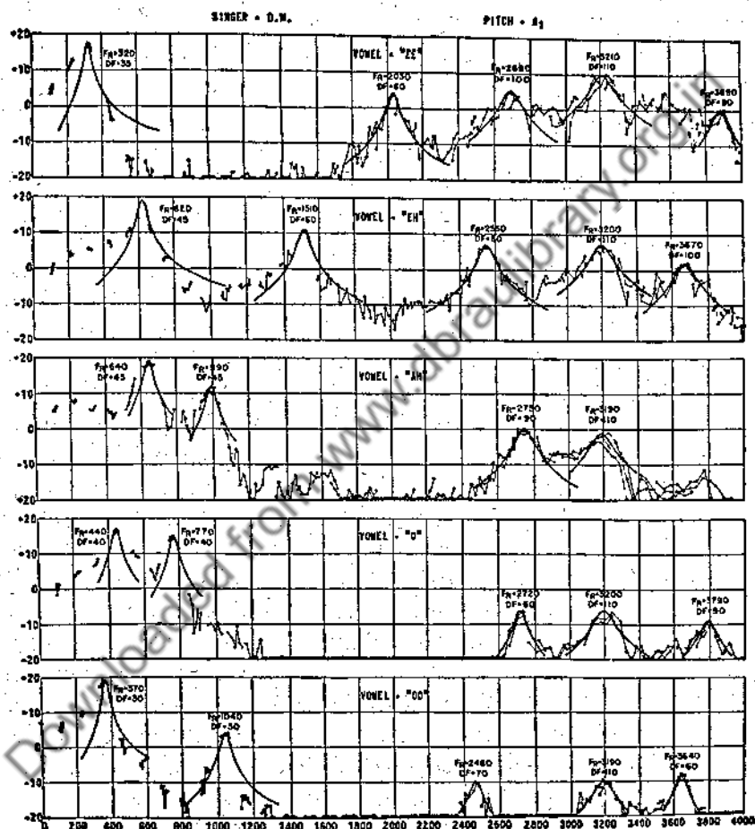
FIG. 6.—Formant regions. (Lewis. 78 )
