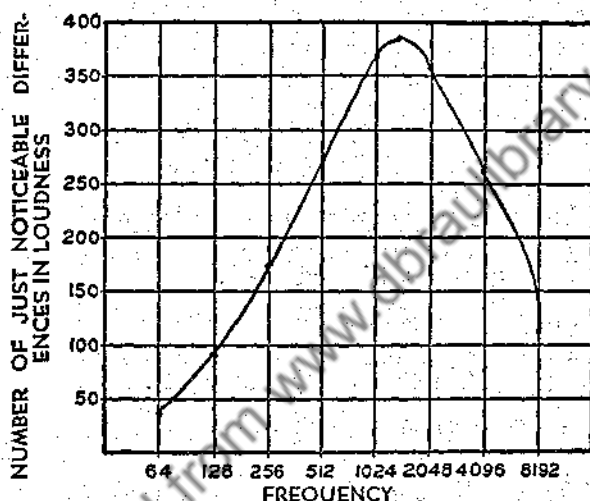
FIG. 4.—The number of just noticeable steps in loudness (j.n.d.) between the threshold of audibility and the threshold of pain. ( Rietz , 112 )
