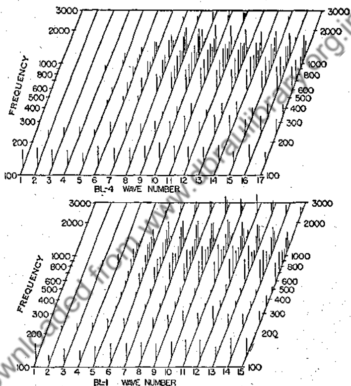
FIG. 4.—Timbre and sonance in a vowel; same vowel spoken twice by the same person. (Black's)
