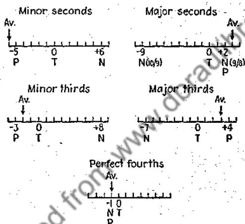
FIG. 17.—Comparison of the tempered and natural scales with the Pythagorean scale. (Greene. 38 )
